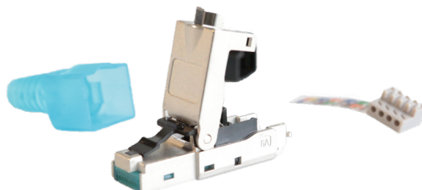
VCR526A/S
